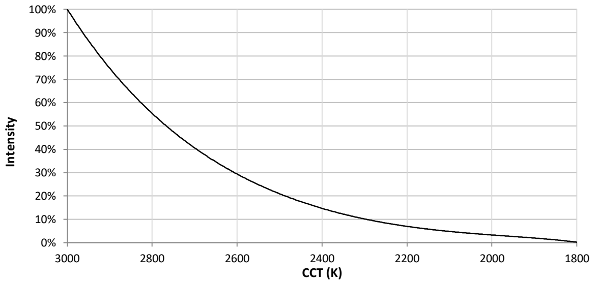
Figure 5: Intensity vs. CCT dimming profile in warm dimming mode
