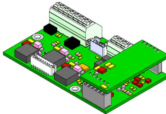
Figure 21: DMX 512-A card plugged in to 0-10V driver board
