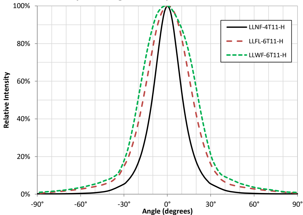
Figure 2: Typical relative intensity over angle
