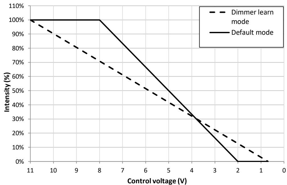
Figure 7: Intensity vs. control voltage in warm dimming mode
