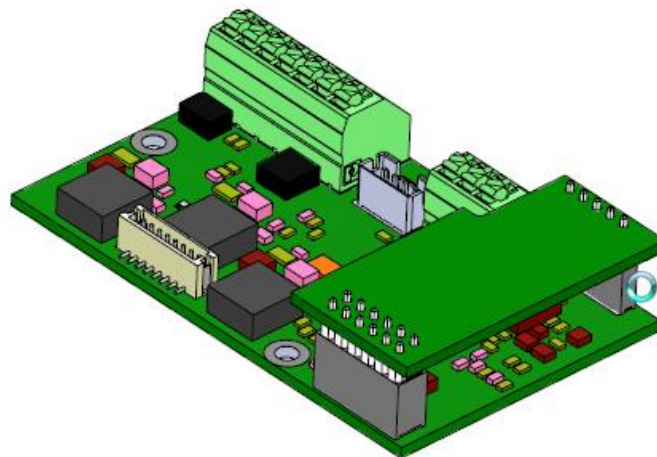
Fig 24. DMX-RDM card connected to 0-10V driver board
