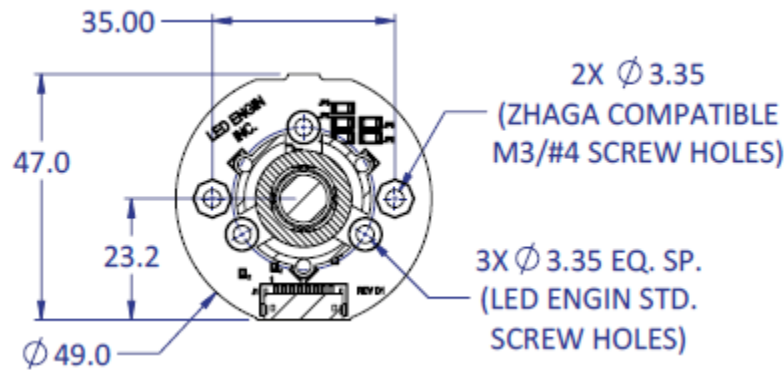
Figure 17: Mounting screw holes in LuxiTune MCPCB
