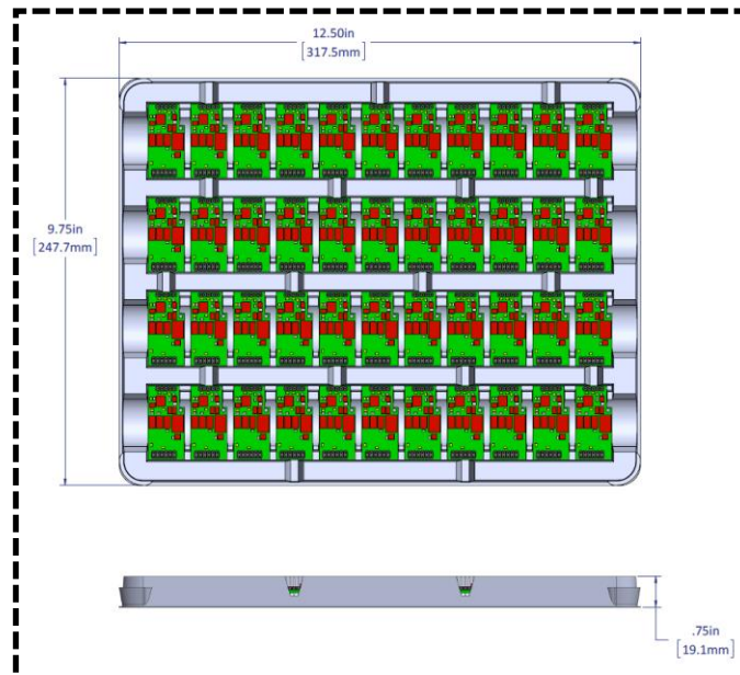
Fig 34: Tray for RDM card
