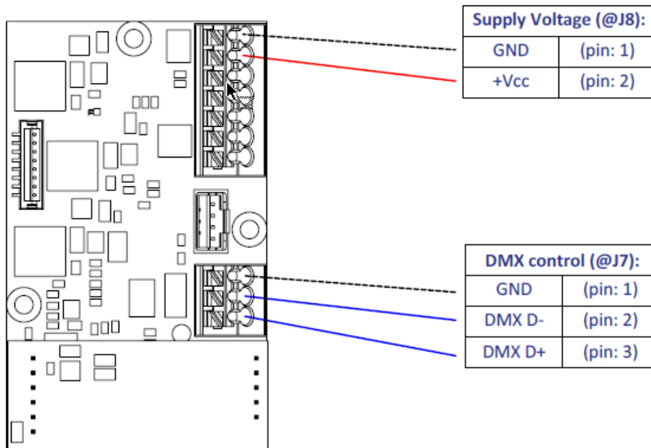
Figure 22: Wiring diagram for DMX control
