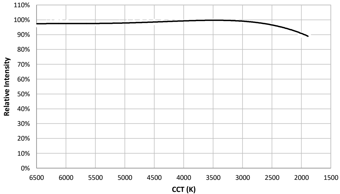
Figure 9: Relative Intensity vs. CCT in CCT tuning mode
