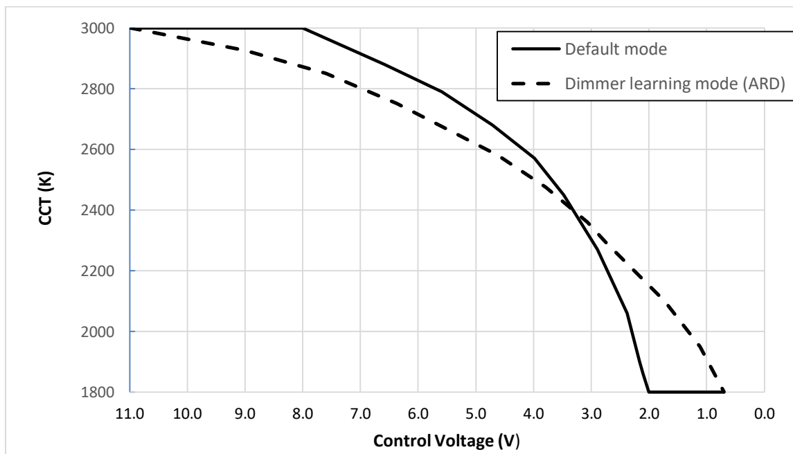
Figure 6: CCT vs. control voltage in warm dimming mode
