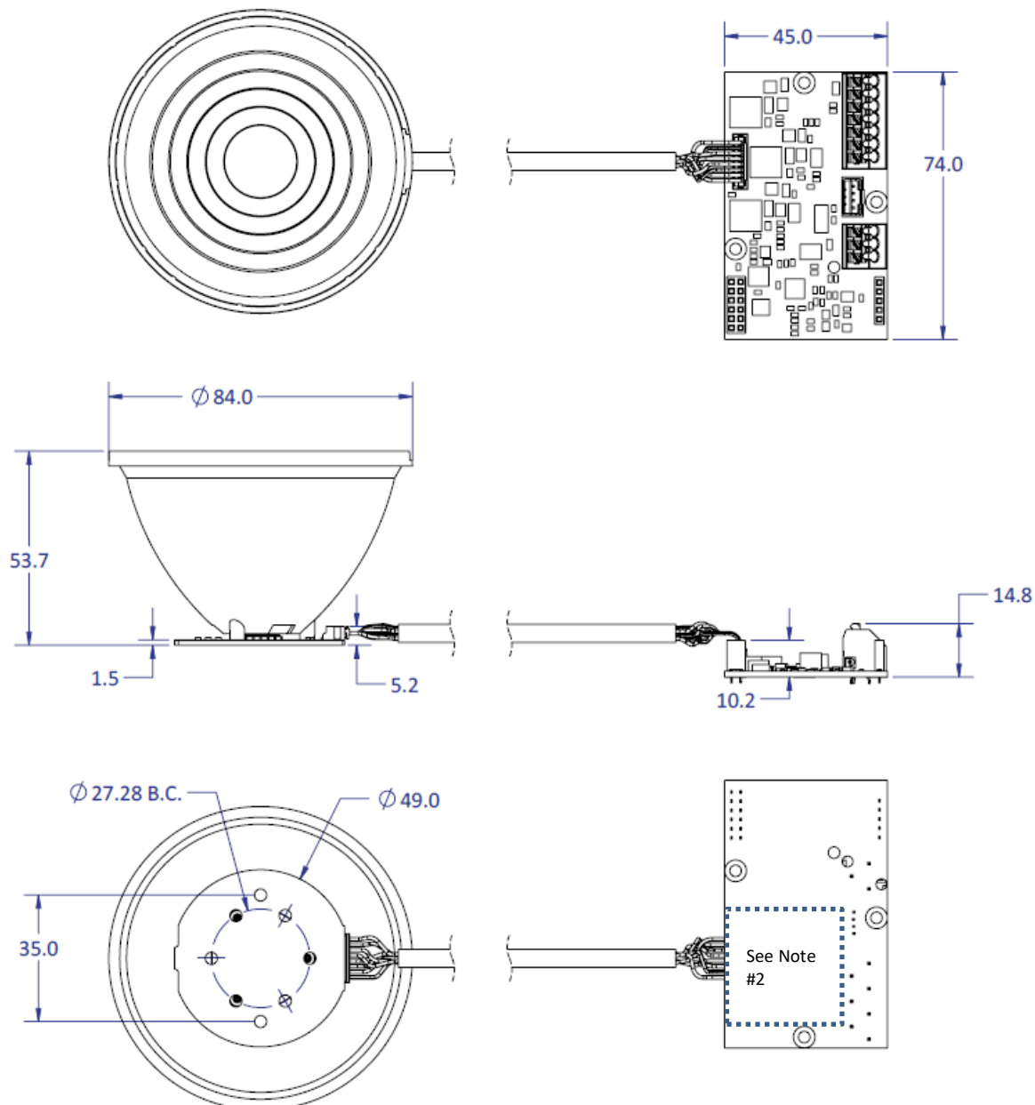
Figure 14: Mechanical dimensions of LuxiTune light engine – with secondary lens
