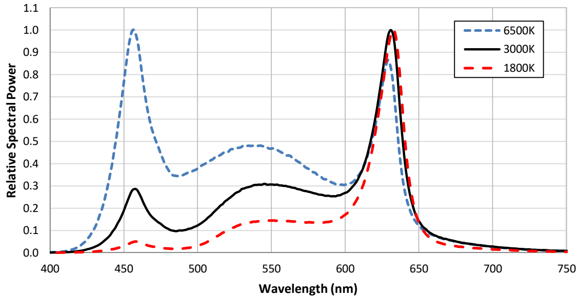
Figure 3: Typical relative spectral power vs. wavelength
