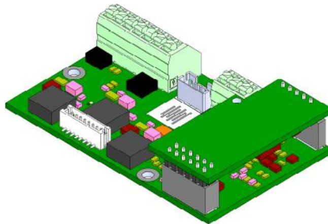
Fig 23. DMX-RDM card connected to 0-10V driver board
