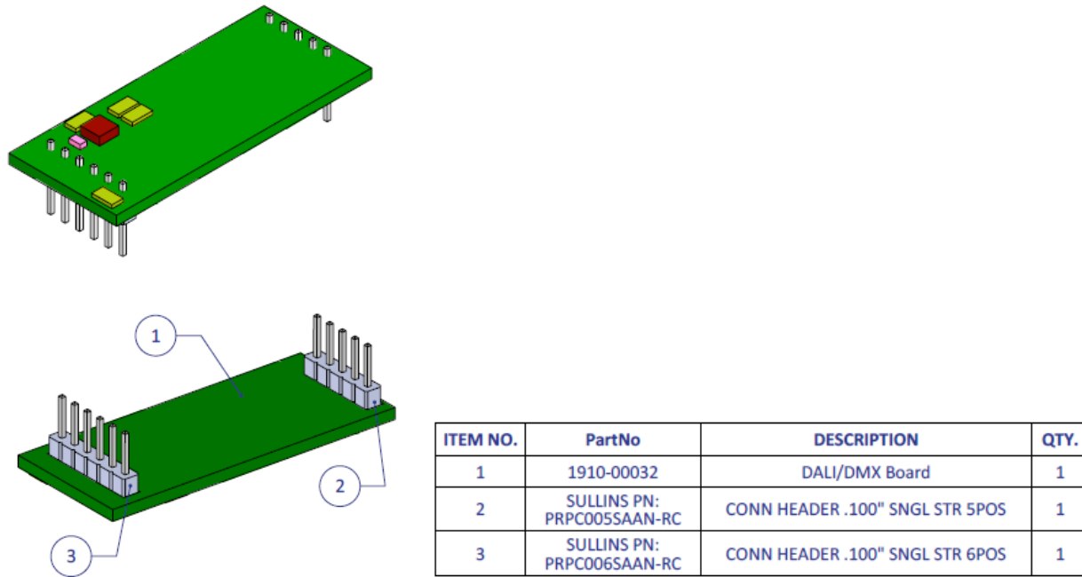
Figure 19: DMX 512-A daughter card
