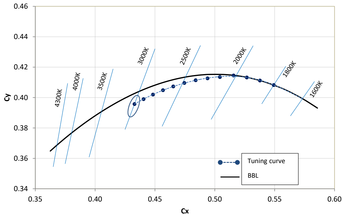
Figure 4: Typical CCT range in warm dim mode
