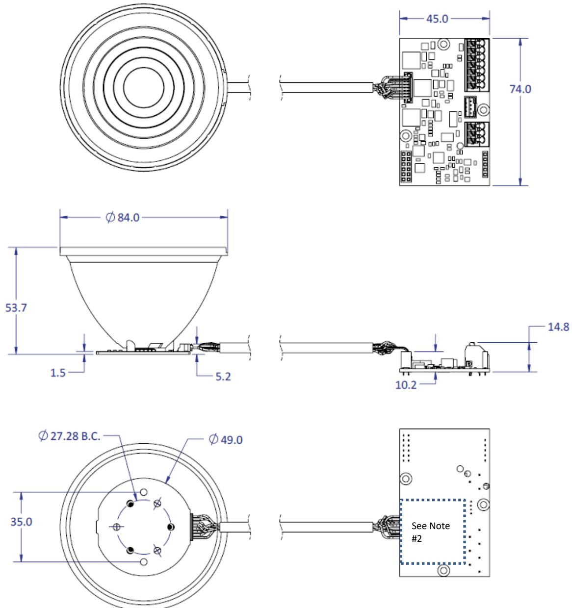
Figure 13: Mechanical dimensions of LuxiTune light engine – with secondary lens
