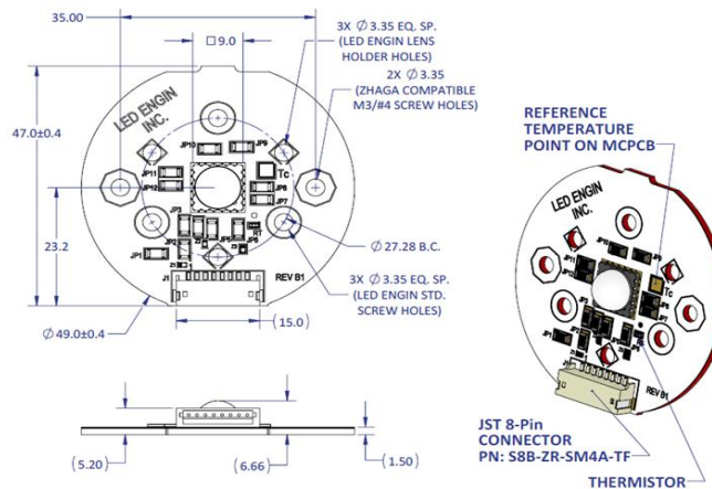
Figure 16: Mounting screw holes in LuxiTune MCPCB
