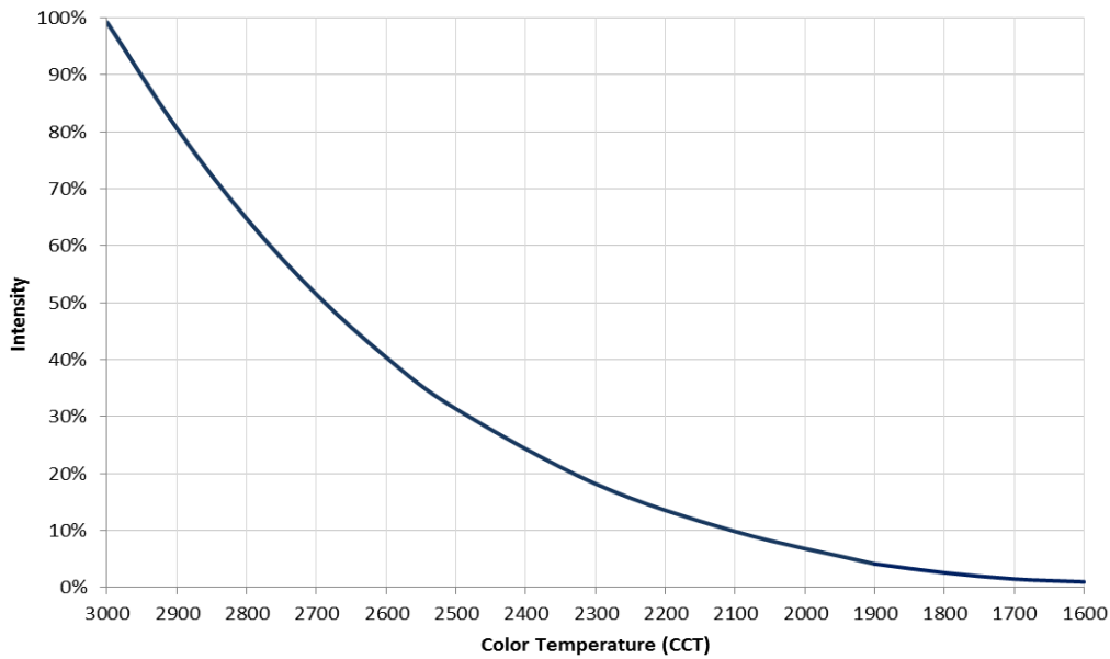
Figure 5: Intensity vs. CCT dimming profile in warm dimming mode
