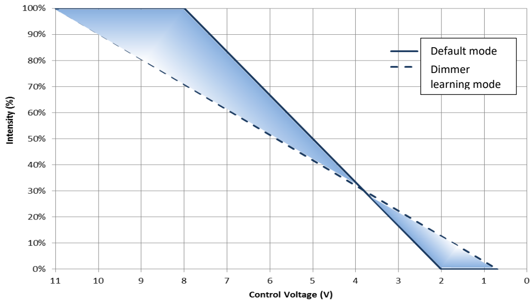
Figure 7: Intensity vs. control voltage in warm dimming mode
