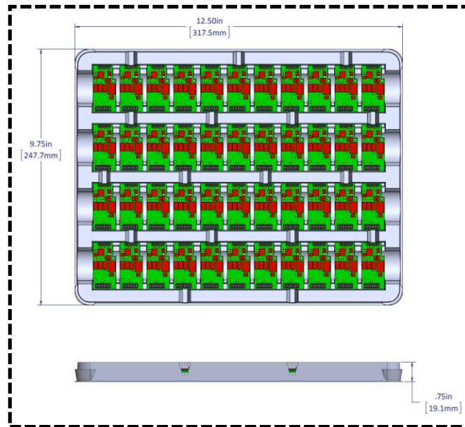
Fig 30: Tray for RDM card
