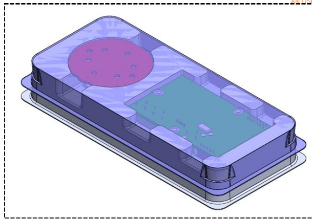
Fig 29. Plastic carrier for LuxiTune units
