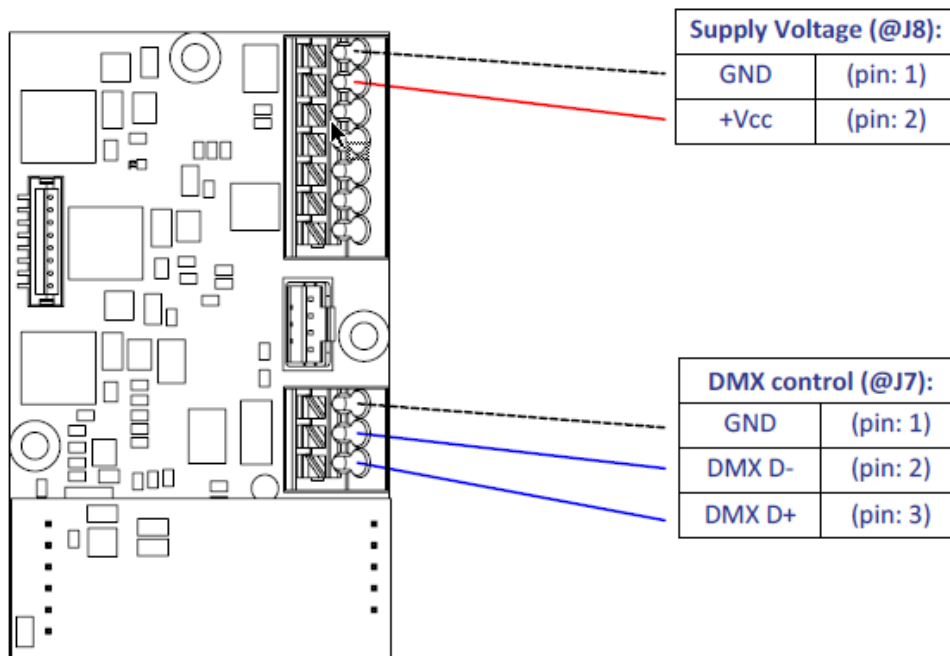
Figure 21: Wiring diagram for DMX control
