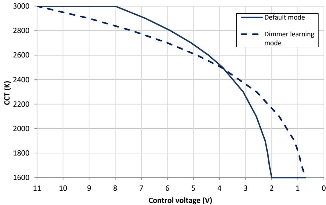
Figure 6: CCT vs. control voltage in warm dimming mode
