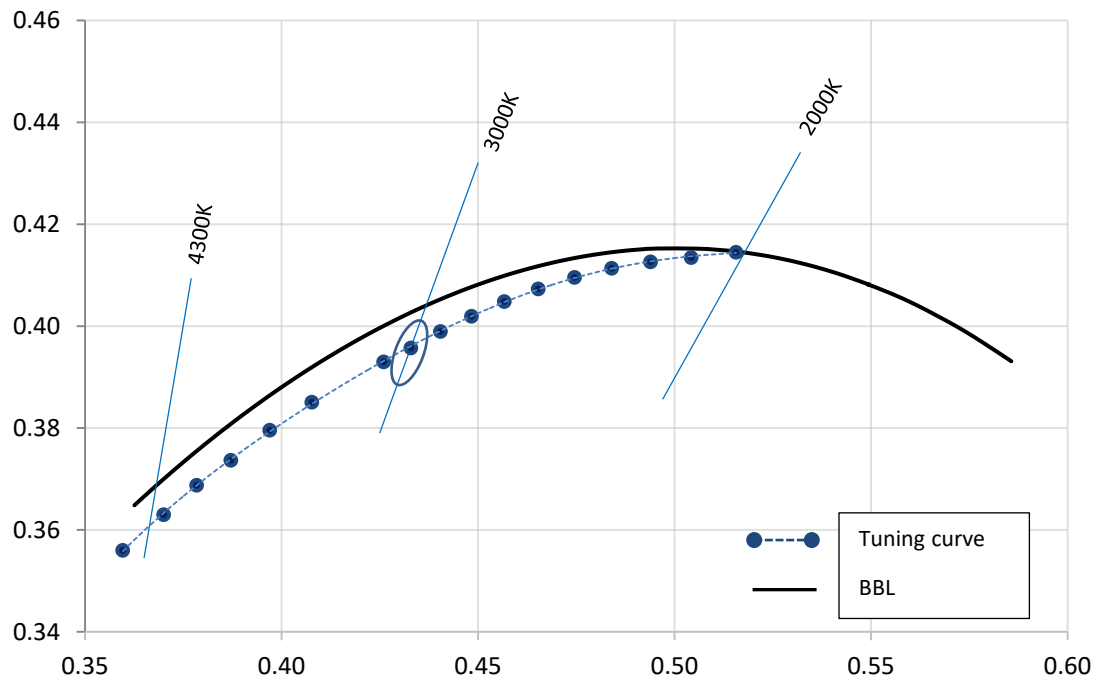
Figure 8: Typical CCT range in CCT tuning mode
