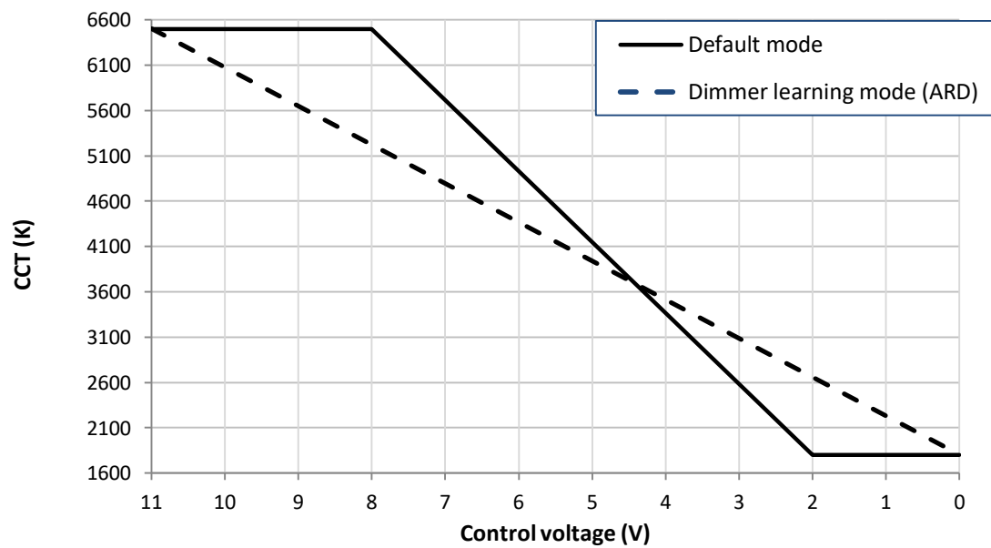
Figure 10: CCT vs. control voltage in CCT tuning mode
