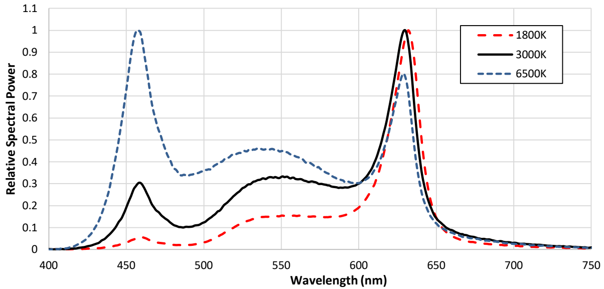
Figure 3: Typical relative spectral power vs. wavelength
