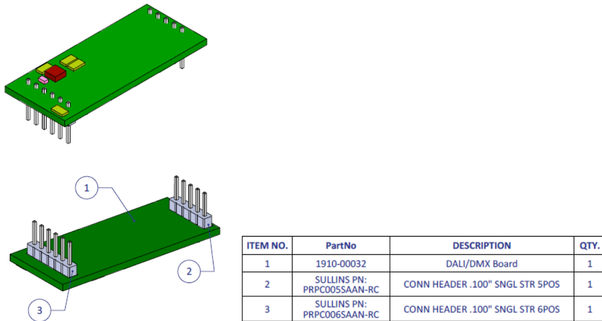
Figure 20: DMX 512-A daughter card
