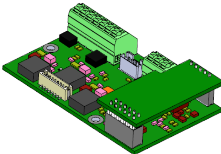
Fig 24. DMX-RDM card connected to 0-10V driver board
