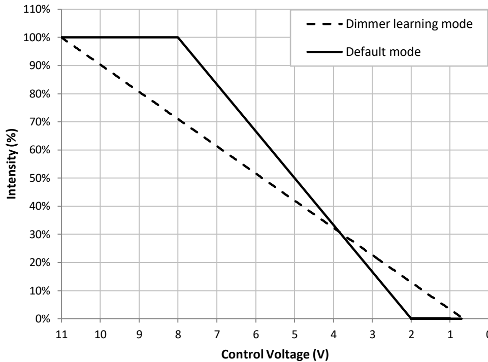
Figure 11: Relative intensity vs. control voltage in CCT tune mode
