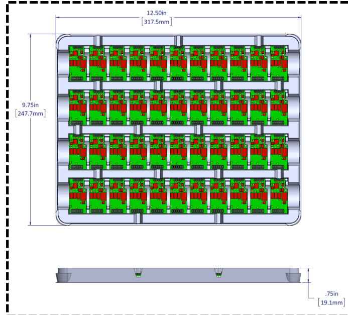
Fig 34: Tray for RDM card
