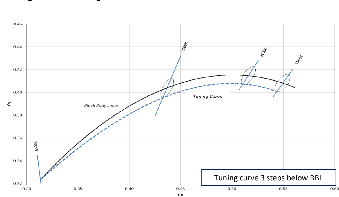
Figure 8: Typical CCT range in CCT tuning mode
