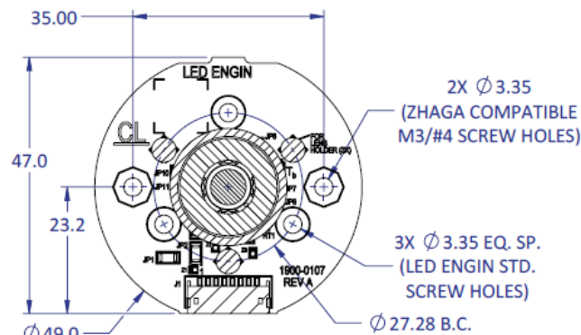
Figure 17: Mounting screw holes in LuxiTune MCPCB
