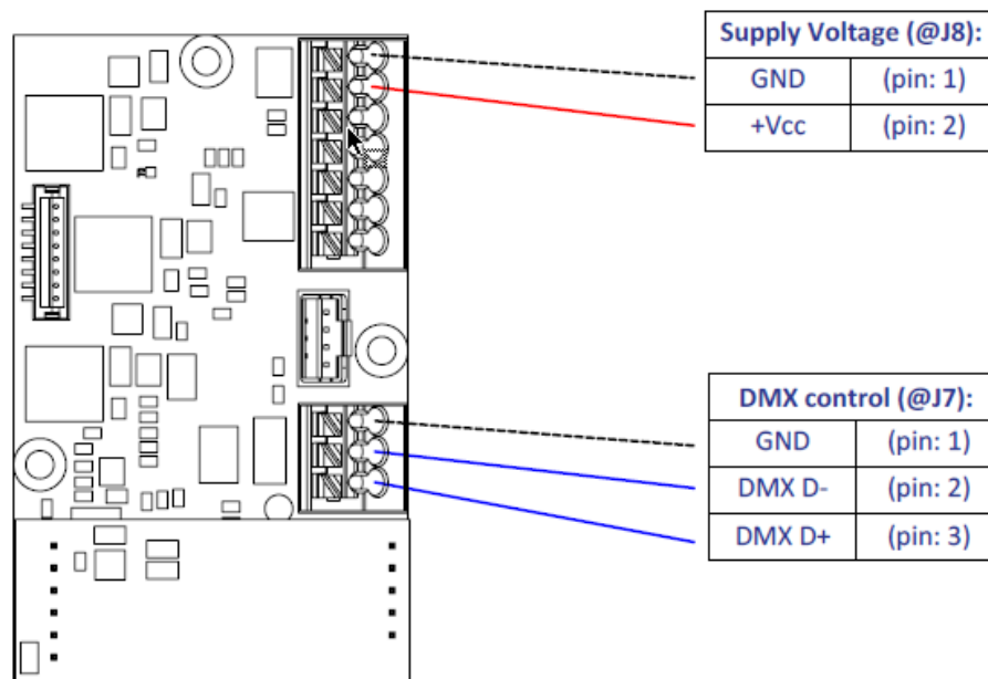
Figure 22: Wiring diagram for DMX 512-A control
