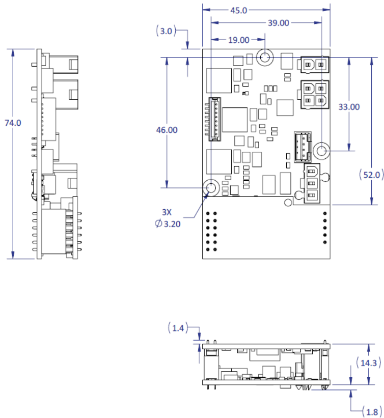
Fig 25. Dimensions of 0-10V driver board with optional DMX-RDM card
