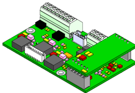
Figure 21: DMX 512-A card plugged in to 0-10V driver board
