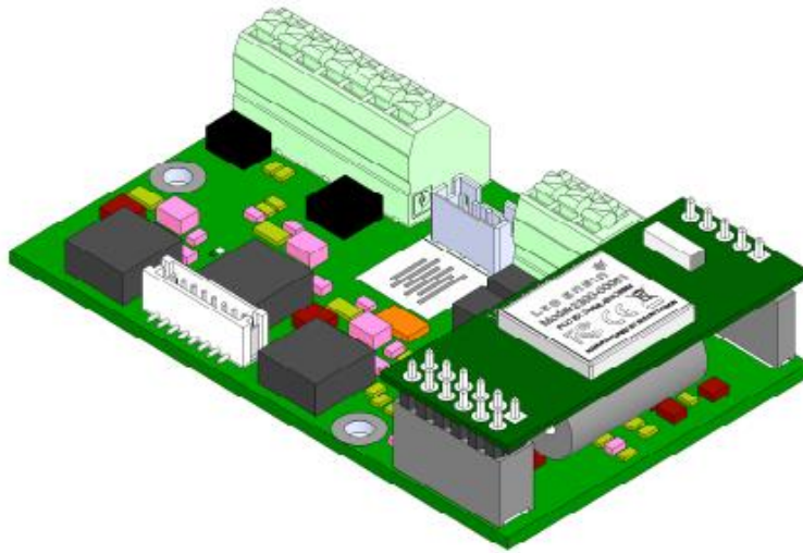
Figure 30: BLE card plugged in to 0-10V driver board
